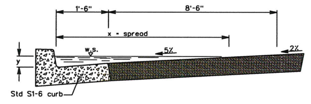
STREET GRADIENT ≥ 6%
