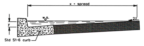
STREET GRADIENT < 6%
